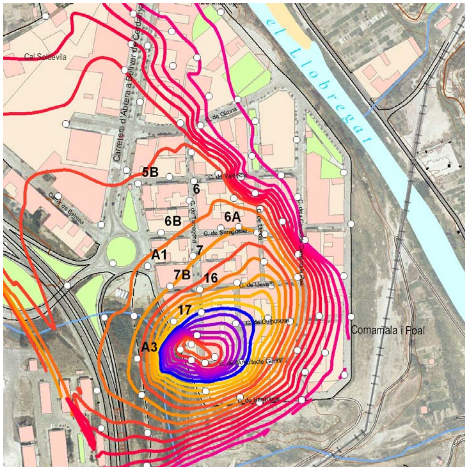
Figure 3 - Subsidence measurements calculated by high topographic levelling.
