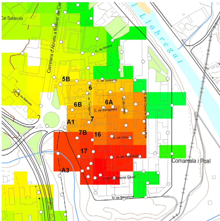
Figure 4 - Subsidence measurements calculated by DInSAR techniques.
