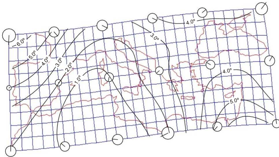
Figure 7- Model results for Dulcert's chart ( w = 0.8 , dmax = 15^\circ , declination as of 1300). The vectors and circles represent displacements from the original; the isolines represent clockwise rotation, in degrees, from the original
