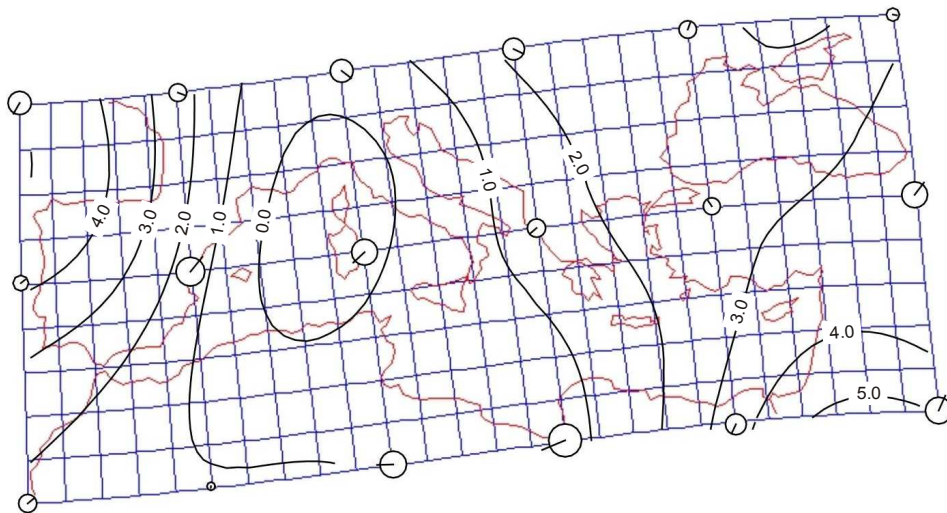
Figure 8- Model results for Aguiar's chart ( w = 0.8 , dmax = 15^\circ , declination as of 1300). The vectors and circles represent displacements from the original; the isolines represent clockwise rotation, in degrees, from the original.
