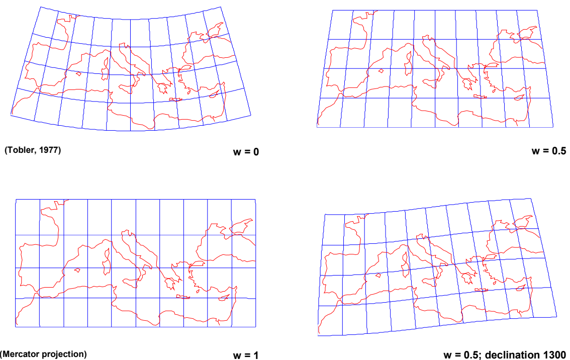
Figure 4 – Test model outputs: w = 0 (only distances: Tobler, 1977); w = 1 (only directions: Mercator projection); w = 0.5 (distances and directions: pseudocylindrical projection); w = 0.5 with magnetic declination as of 1300.
