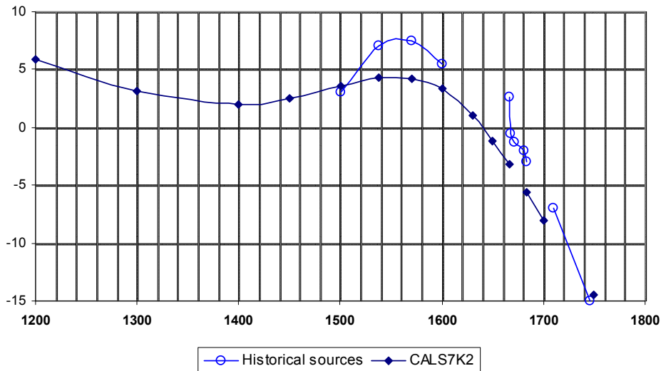
Figure 10 – Variation of the magnetic declination in Lisbon. Comparison between the geomagnetic model CAL57K2 by Korte and Constable (2005) and some observed values 13 . Horizontal axis: years; vertical axis: declination (degrees).
